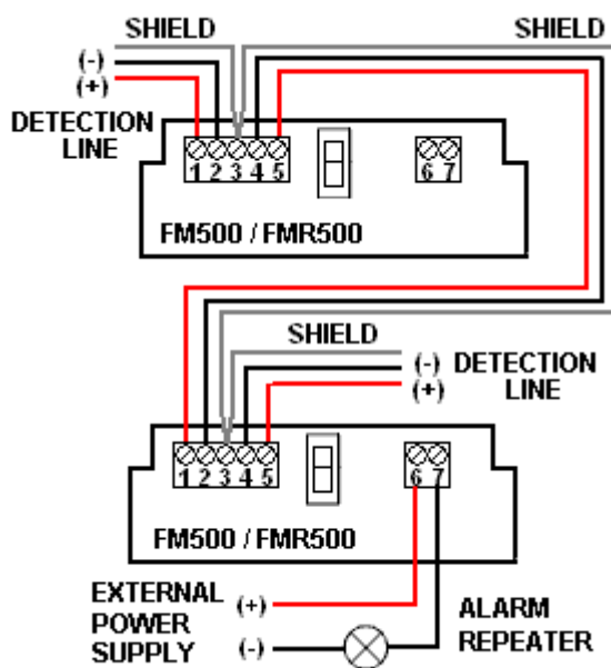
Fig. 3 – Connection diagram
