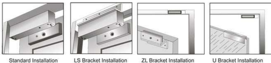
Standard Installation
